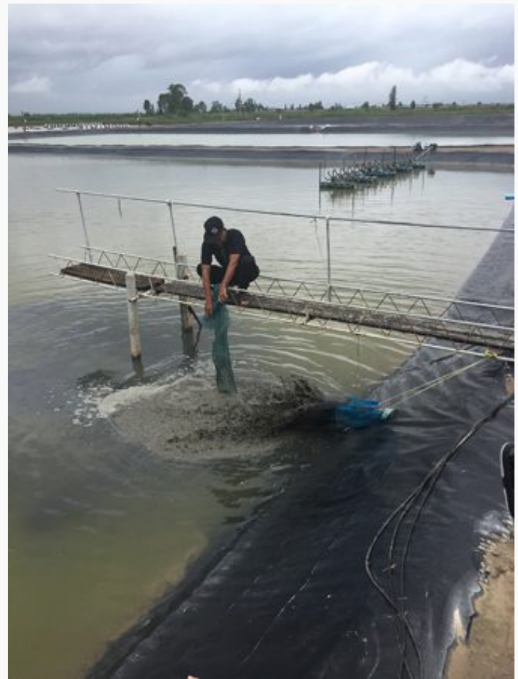
Draining effluent from a central drain in the growout pond to a sedimentation pond two hours after feeding the shrimp.
